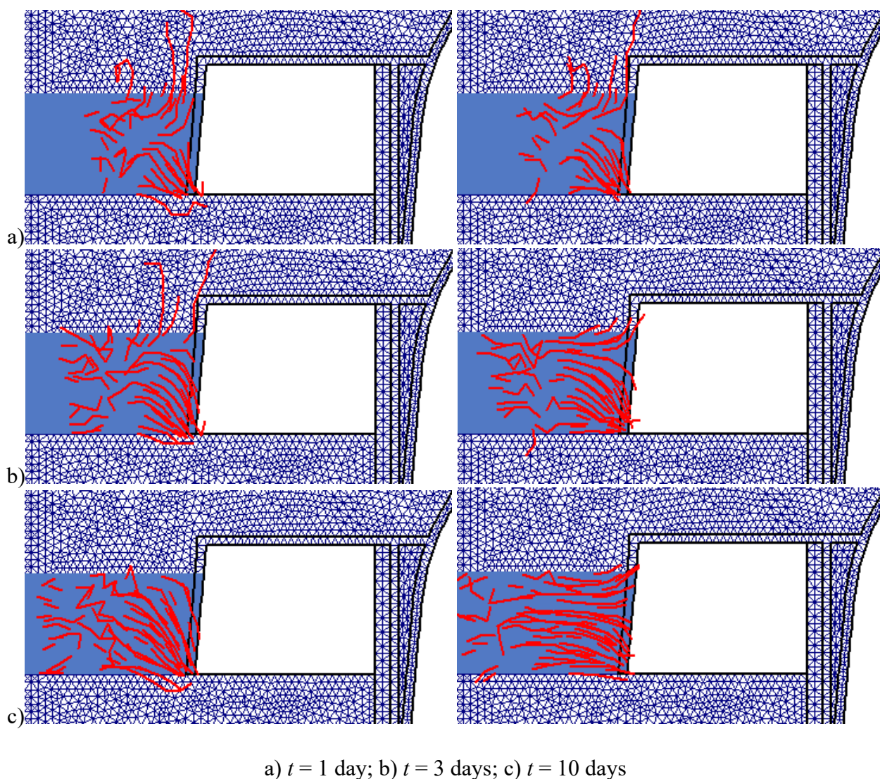
Figure 7 – Trajectories of methane filtration: H = 400 m (left side); H = 1000 m (right side)
